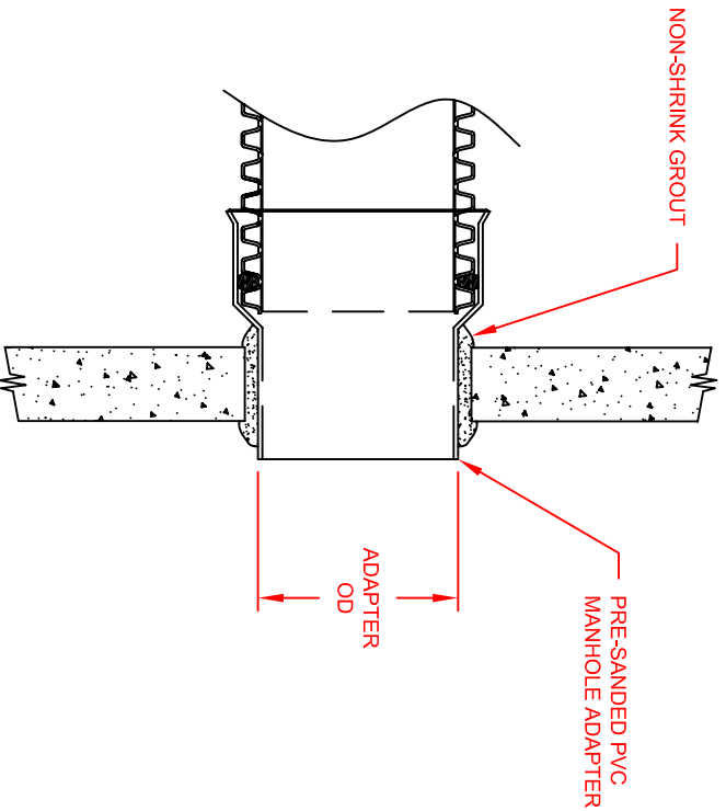
TYPE 2: SANDED PVC MANHOLE ADAPTER GROUTED INTO MANHOLE WALL
