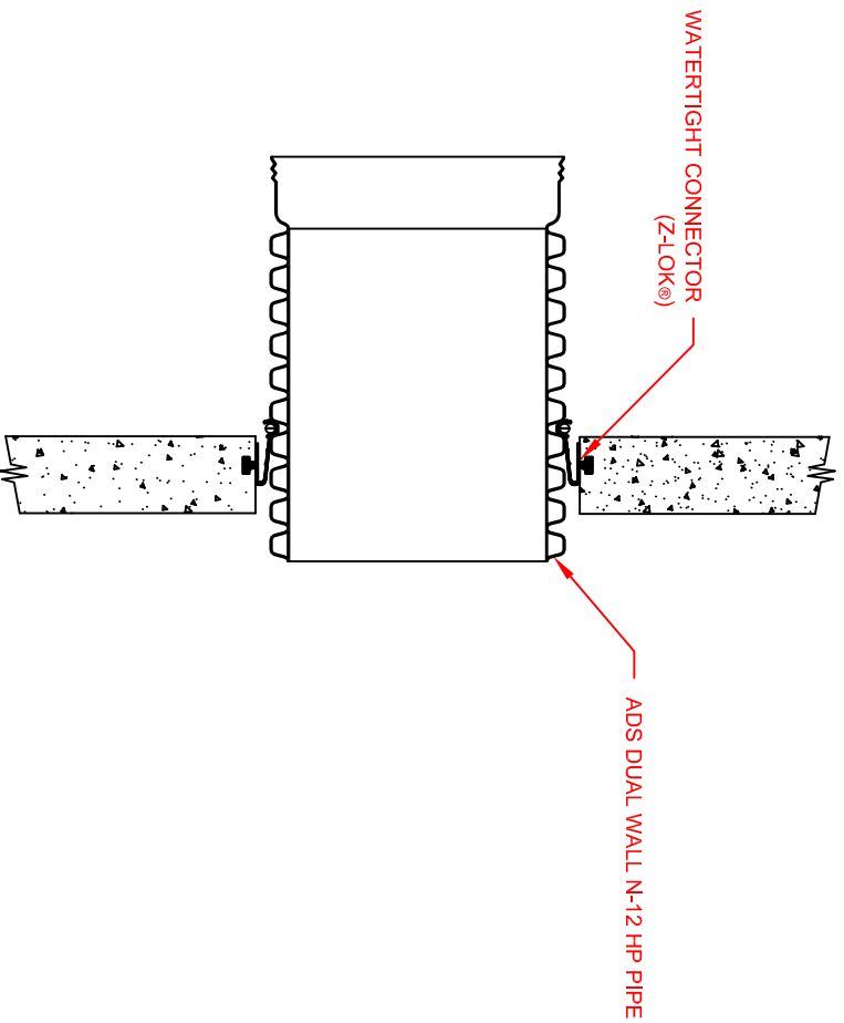
TYPE 4: Z-LOK (PRE-CAST MANHOLE GASKET) SECURED DIRECTLY TO EXTERIOR PIPE CORRUGATIONS
